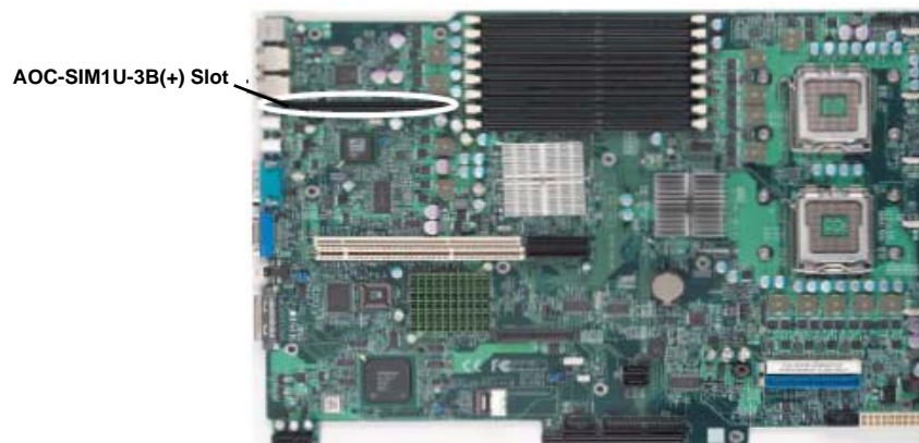
Figure 2-8. X7DBX/X7DBX-i Series
