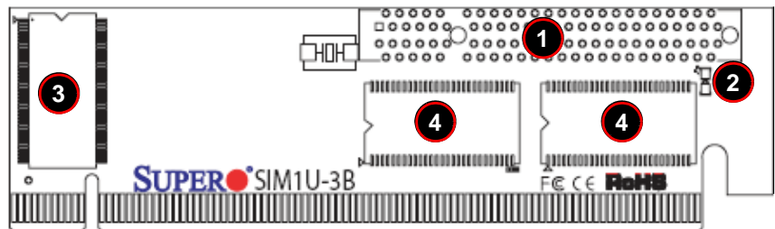
Figure 2-3. AOC-SIM1U-3B/3B+ Add-on Card – Rear View
