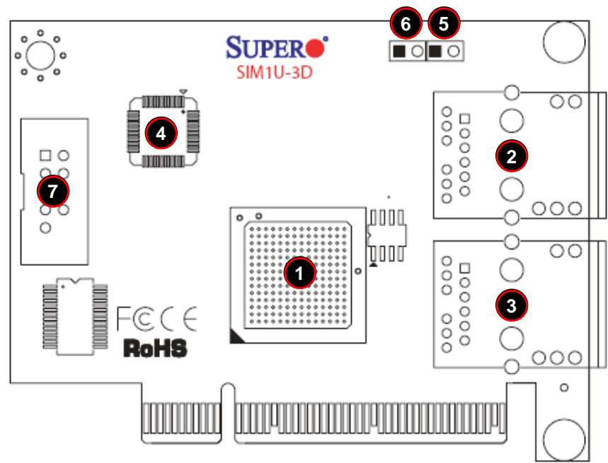
Figure 2-4. AOC-SIM1U-3D Daughter Card
