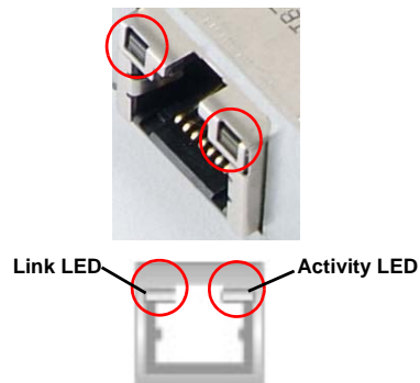
Figure 2-6. AOC-SIM1U-3D Daughter Card LAN LED Indicators
