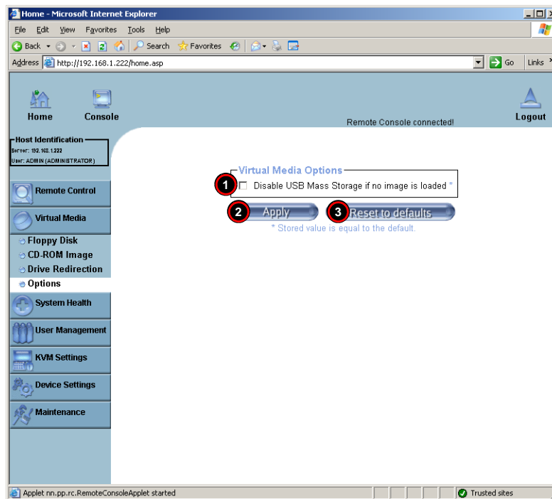
Figure 3-9. Virtual Media Options Screen
