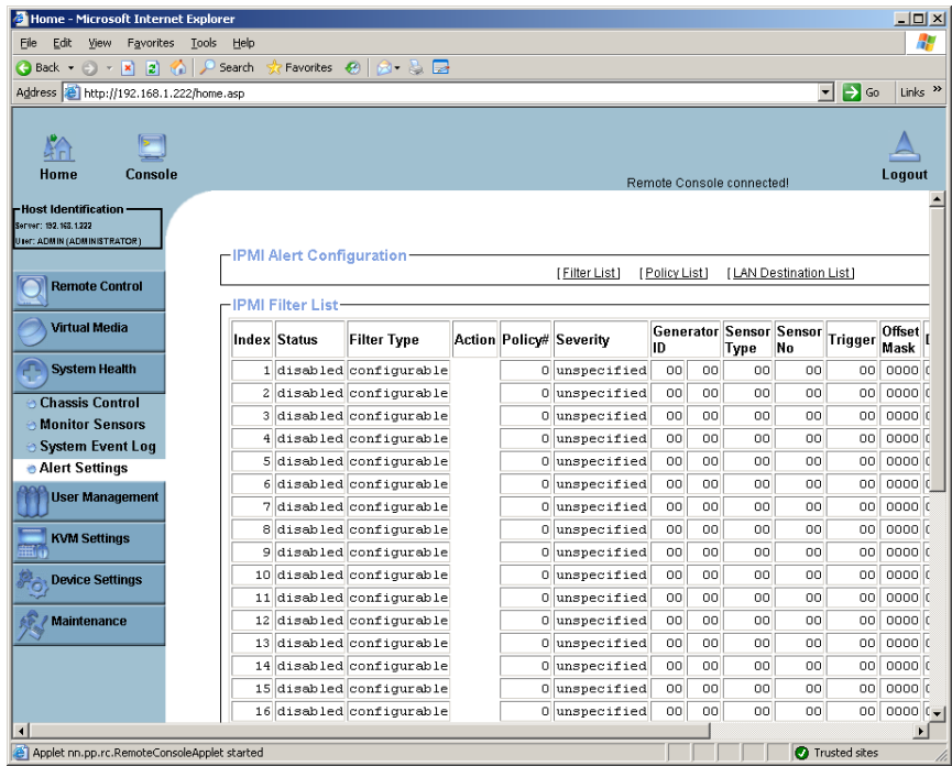
Figure 3-13. Alert Settings Screen
