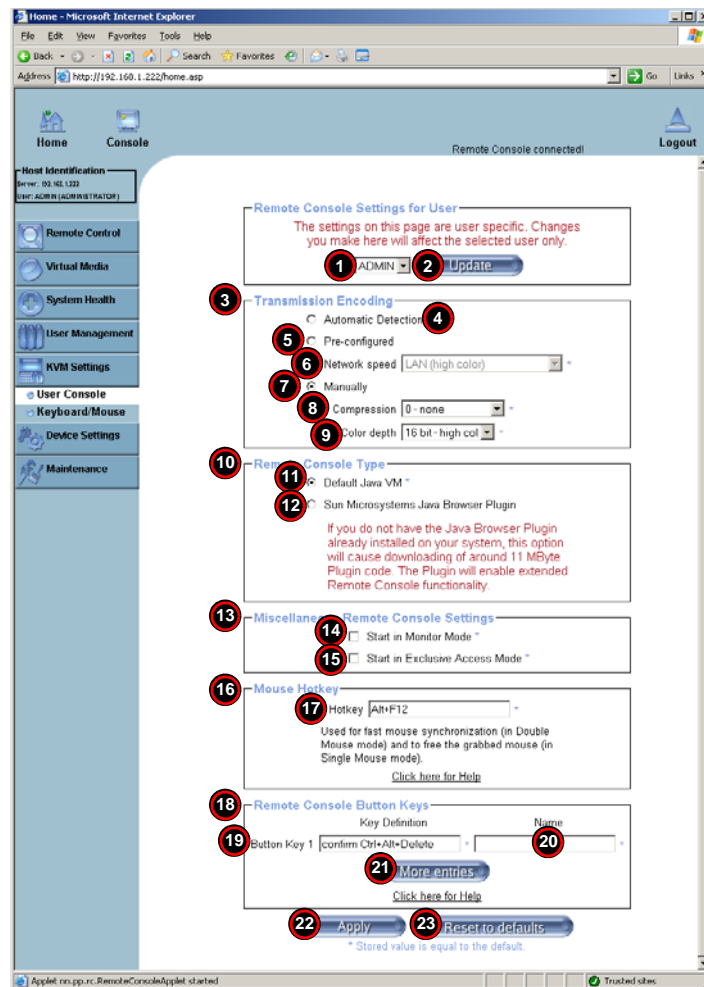
Figure 3-17. User Console Screen
