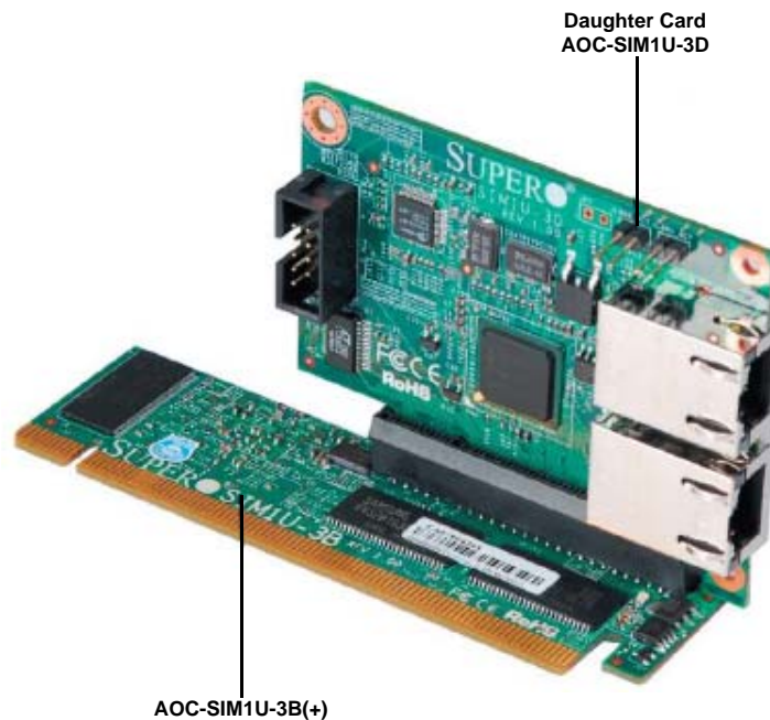
Figure 2-1. AOC-SIM1U-3B/3B+ Add-on Card Connected to AOC-SIM1U-3D Card
